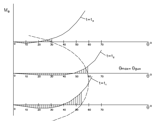
Figure 2. Transverse stability diagram in different moments of time.
